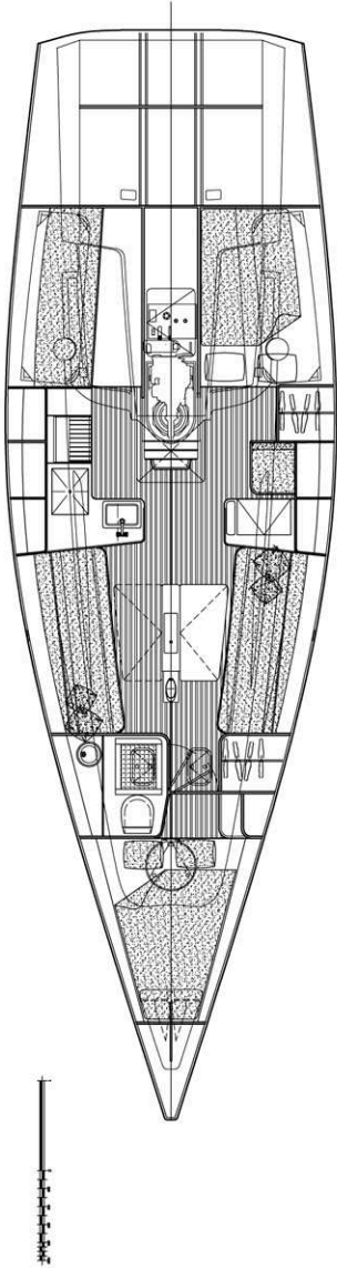
Open Aft Cabin Option 1:30
